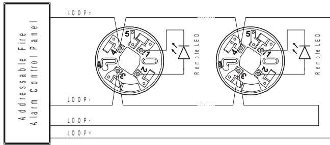
Figure 1. Wiring diagram:
